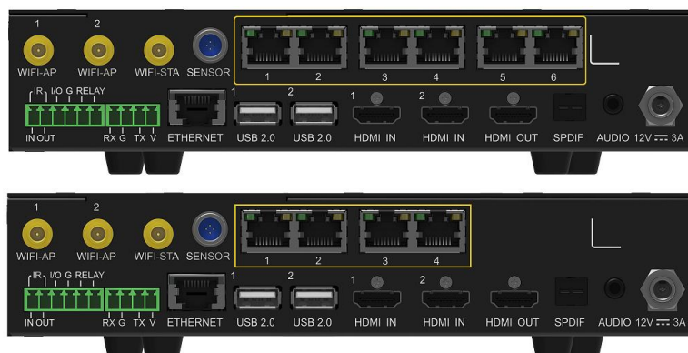
Figure 2-2 Rear panel – TU20 Pro (6 Ethernet ports) / TU15 Pro (4 Ethernet ports)
