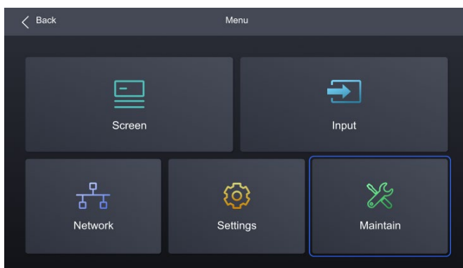
Figure 4-3 Main menu
